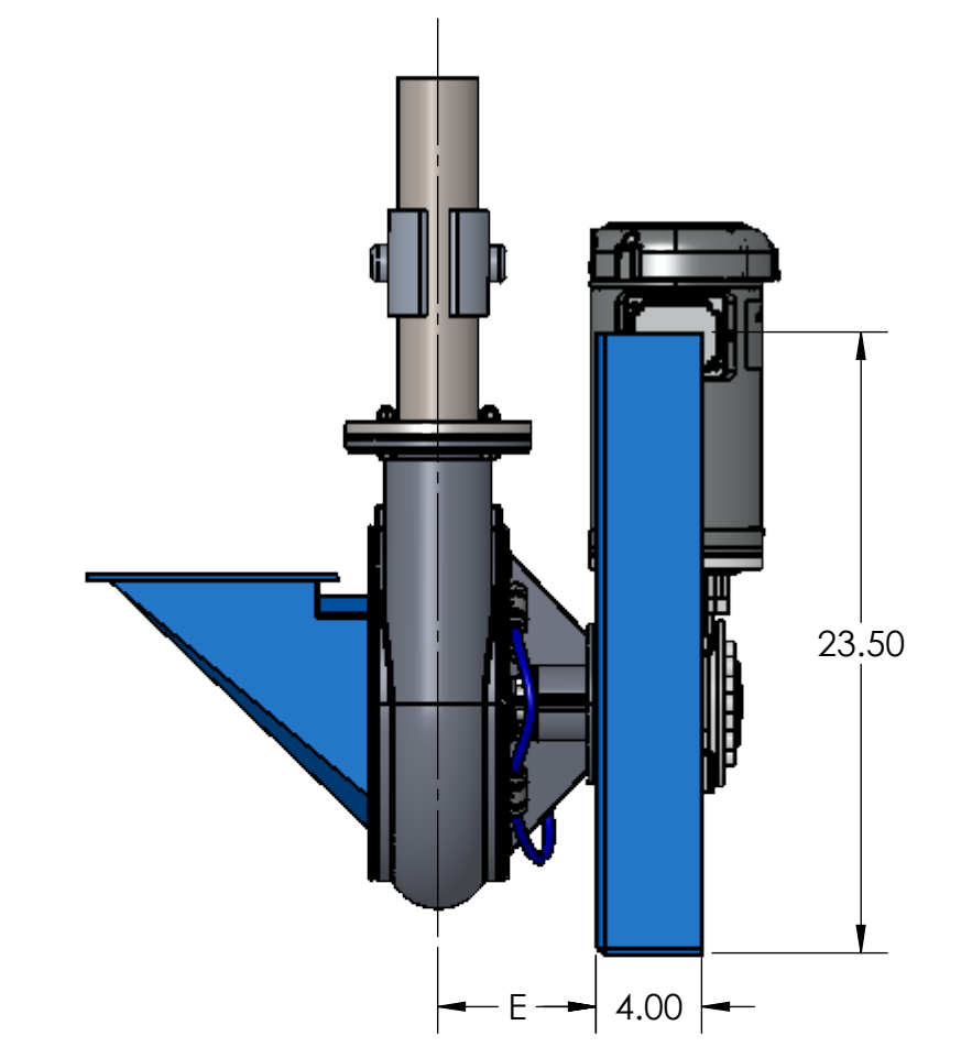
BOTTOM DRIVE DETAIL (OPTIONAL)
