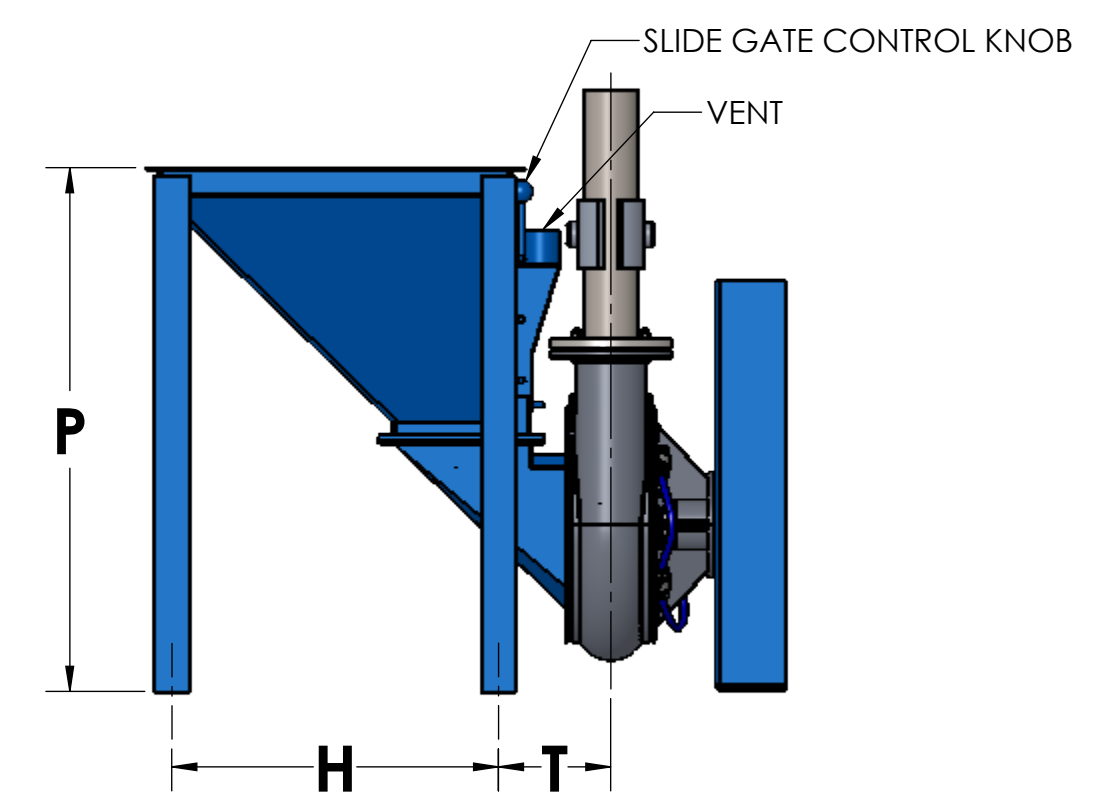
STANDARD CHARGE HOPPER DETAIL 1.50 CU. FT. CAPACITY (OPTIONAL)
