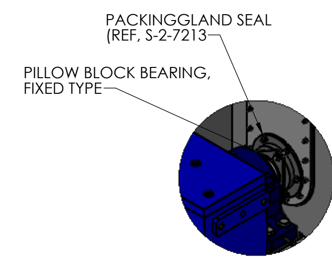
DRIVE SIDE DETAIL *NOTE STIFFENER HIDDEN TO SHOW DETAIL*
