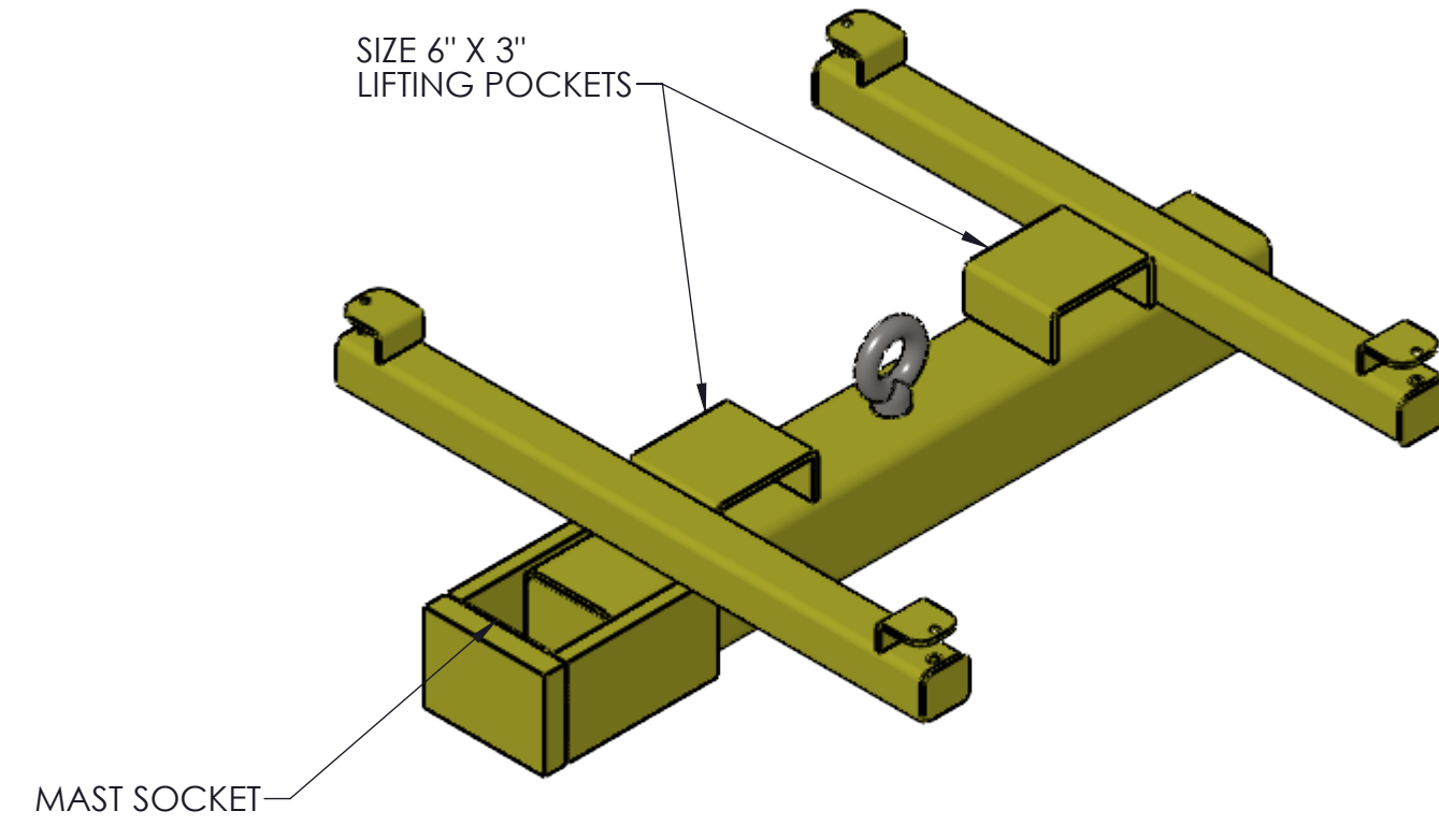
REMOVABLE LIFTING BRACKET 3000 LB LOAD CAPACITY
