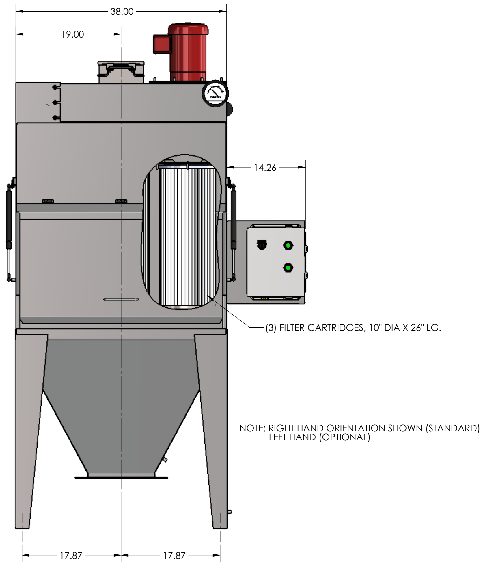
VIEW SHOWN WITHOUT CHARGE DOOR FOR CLARITY
